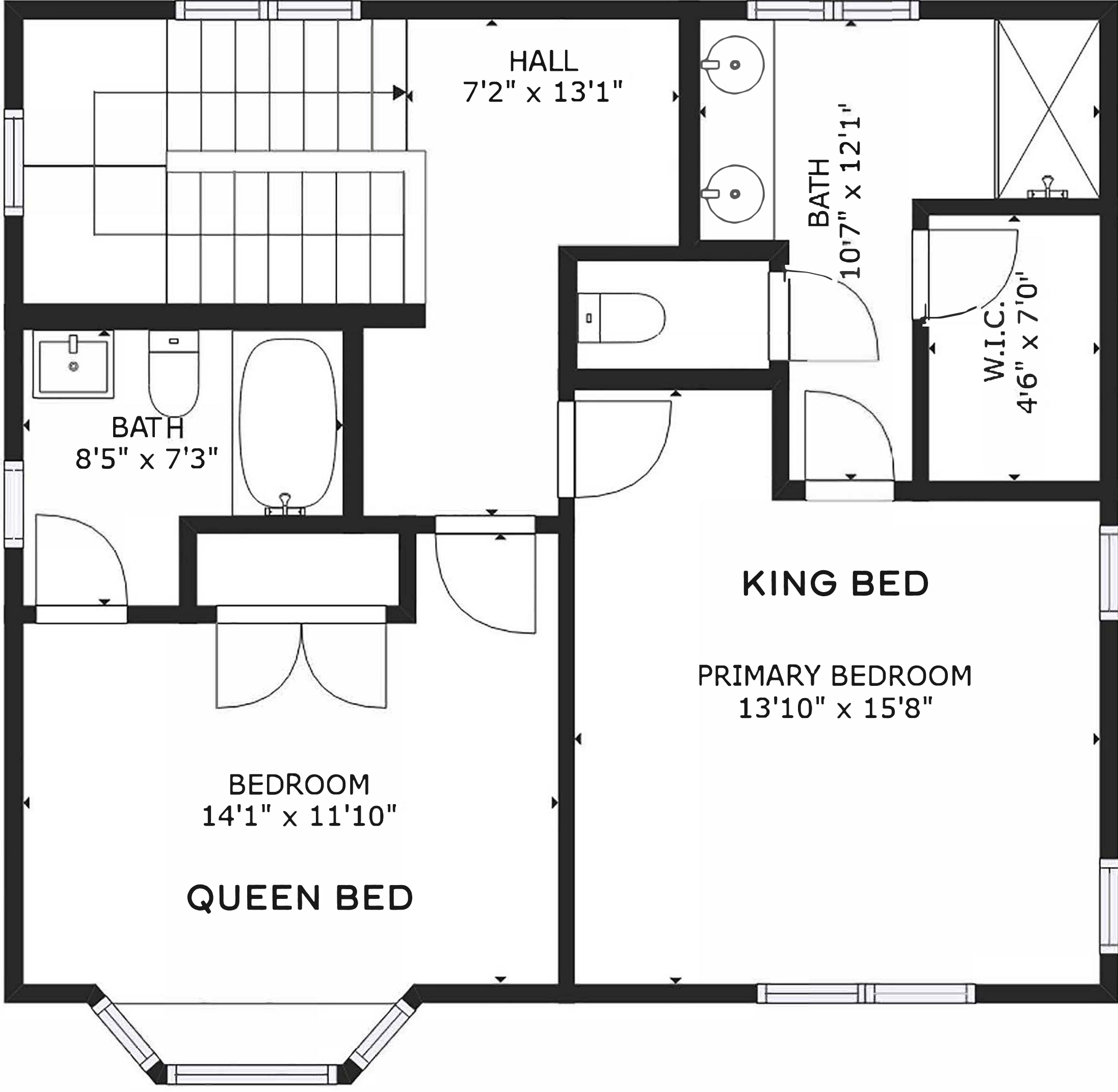
FLOOR 3
